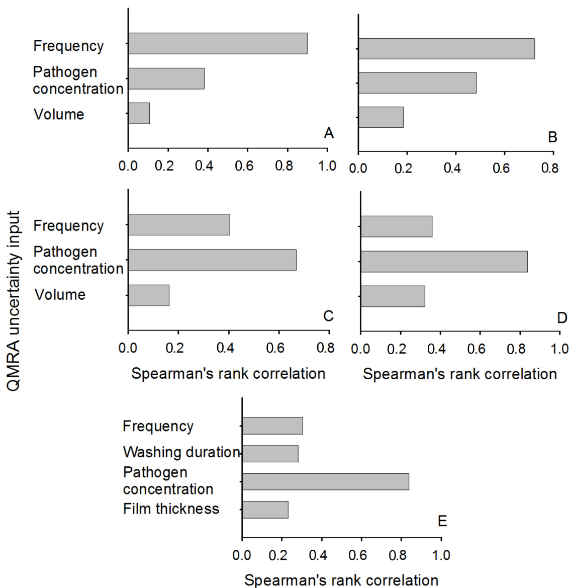
Figure 4. Uncertainty as determined by Spearman's rank correlation for each worst-case scenario using Shigella spp. as the representative bacteria. (A) Scenario (i)—accidental ingestion (drinking); (B) Scenario (ii)—aerosol exposure; (C) Scenario (iii)—garden work; (D) Scenario (iv)—crop consumption; and (E) Scenario (v)—handwashing.
