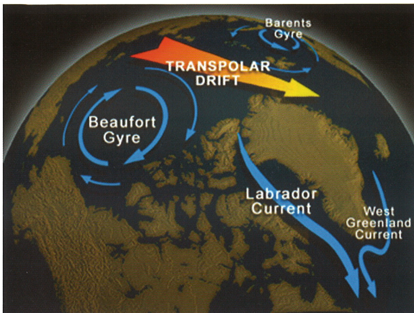
The main currents of the Arctic Ocean. During periods of high AO index, the Beaufort Gyre weakens, and divergent ice is entrained into the Transpolar Drift Stream, where it is exported from the Basin east of Greenland.
