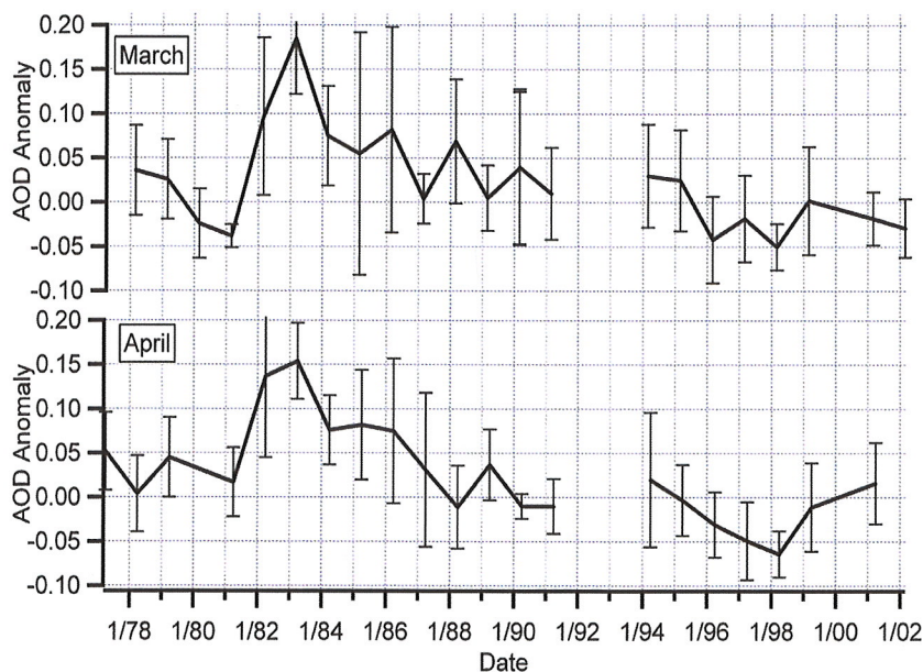
Monthly averaged aerosol optical depth anomalies at Barrow, Alaska, for March and April. The anomalies are relative to a base of non-volcanic years. The data from 1992 and 1993 were removed because of stratospheric aerosol influx from the Mount Pinatubo eruption in 1991. The vertical lines represent one standard deviation of the monthly mean. The data were made available by NOAA CMDL.
