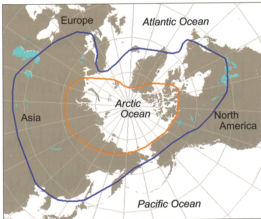
Range of the Arctic air mass in winter (January, blue) and summer (July, orange).
