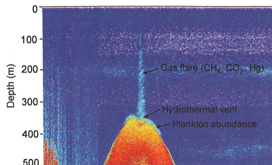
Gas plume venting from the Piips volcano.
