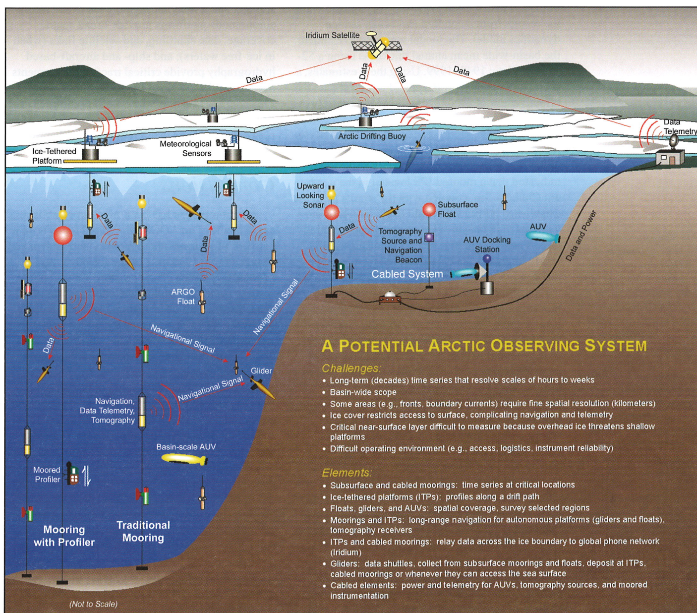
Components of the Arctic Ocean Observing System (AOOS).
