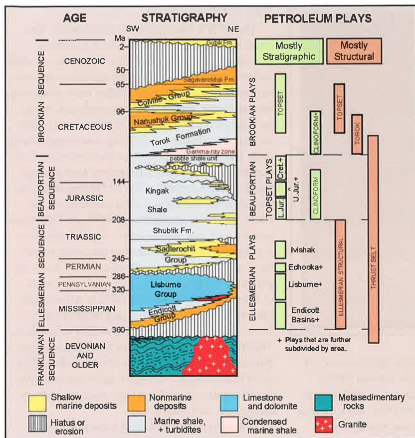
Ages, names, and rock types present in NSP. The colored bars on the right show the stratigraphic position of the 24 petroleum plays evaluated in the 2002 assessment. Note that the bars with a "+" symbol indicate multiple plays in different areas. Plays indicated by bold outlines include those with the greatest oil and/or gas potential.
