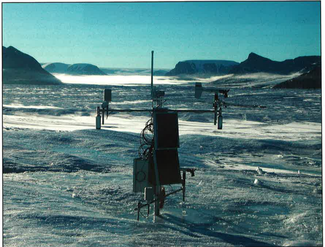
Automatic weather station at Petermann Glacier (part of a joint project with the National Science Foundation described in the NSF section).
